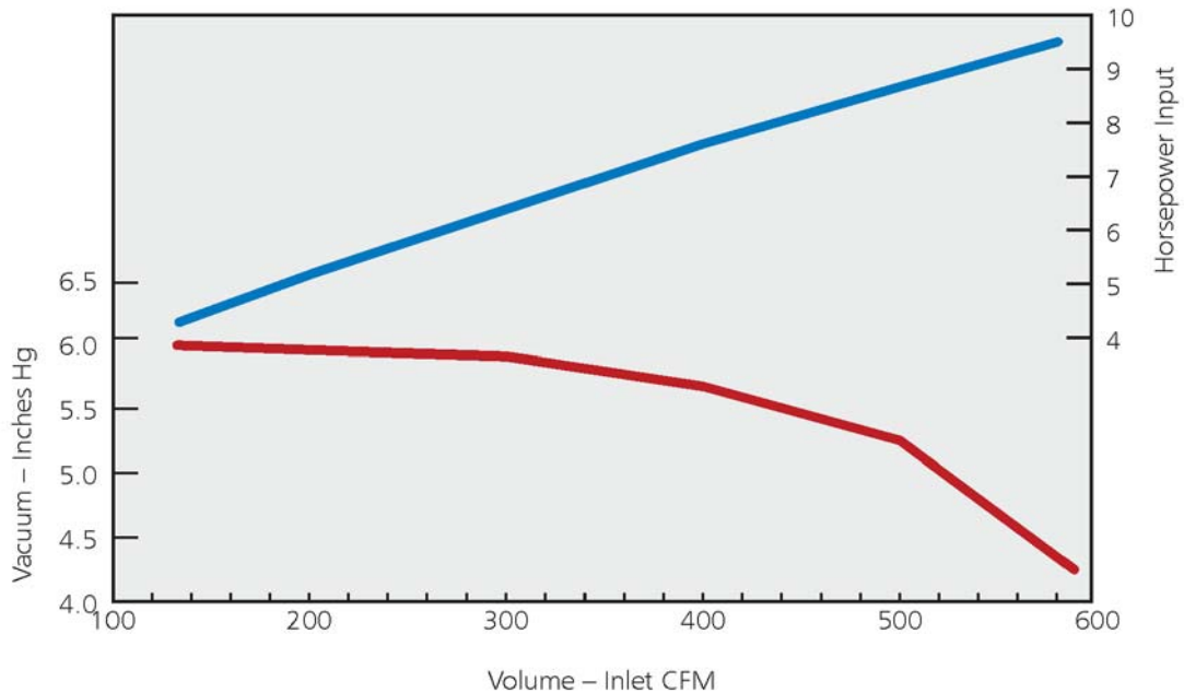
Chart 4 Gardner Denver Performance Curve Model 407 Atmosphere Conditions 29.92 inches Hg 68°F
